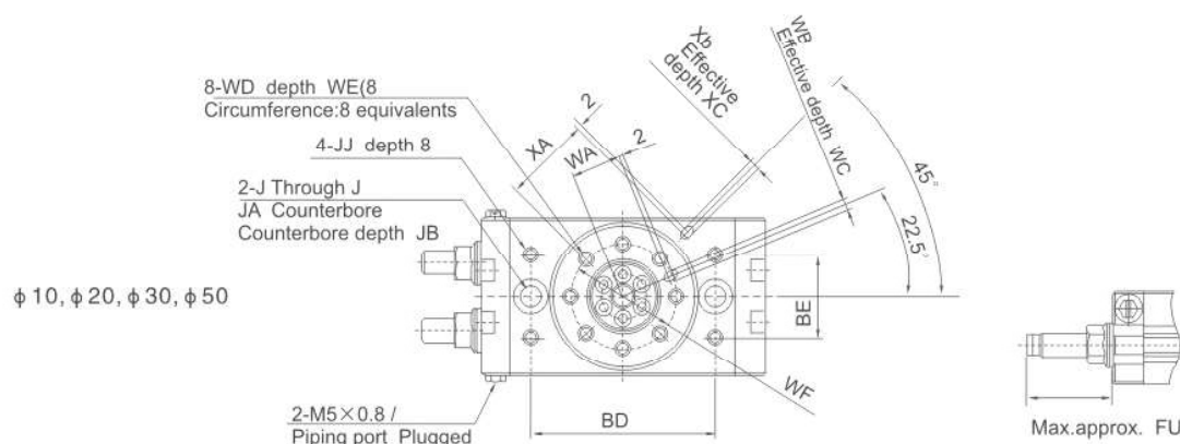
Basic style: MAQB□A
