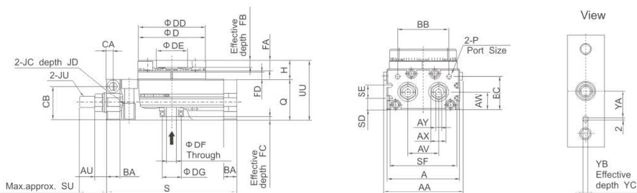
With internal shock absorber MAQB□R
